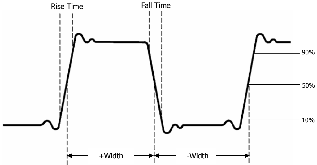
Figure 2-112 The time parameters
