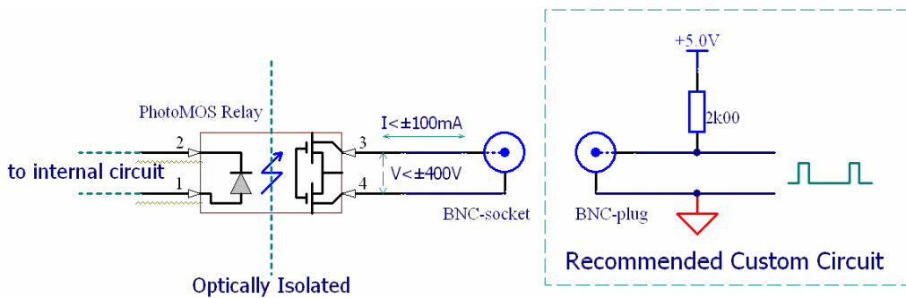
Figure 2-91 Schematic Diagram of Pass/Fail output
