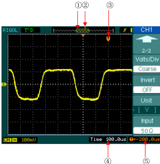
Figure 2-32 Marks indicator
