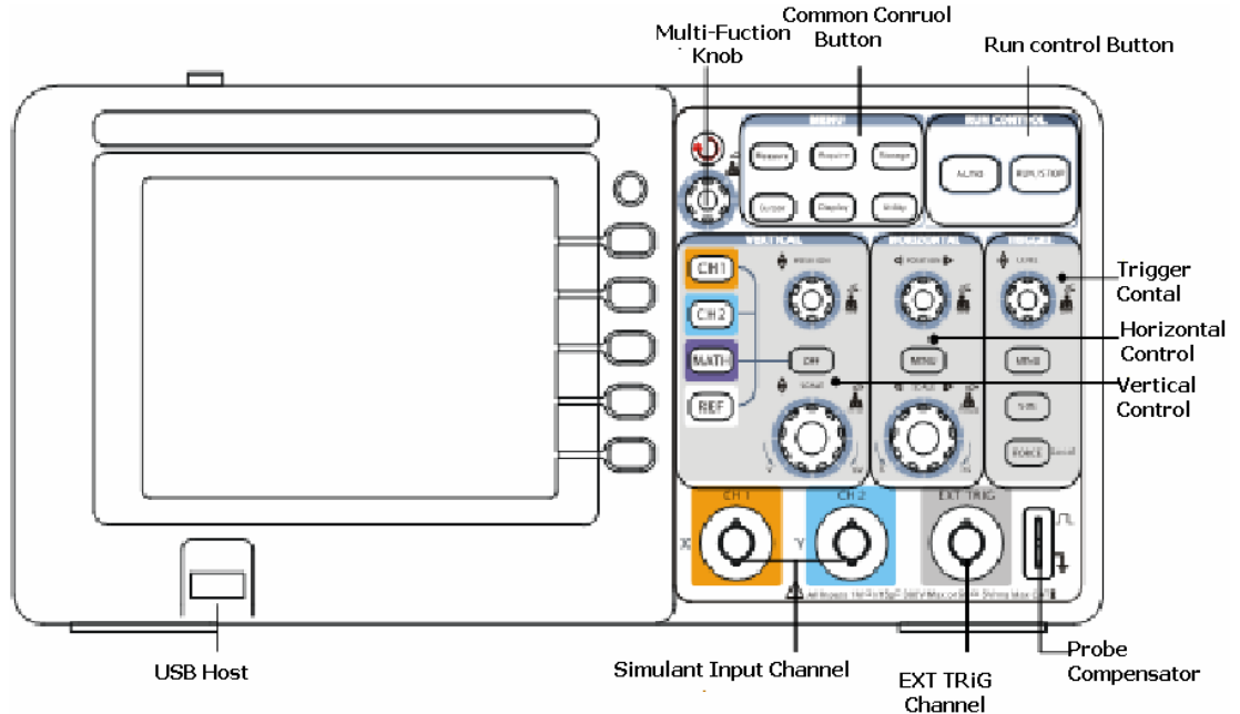
Figure 1-2 Front Panel Controls
