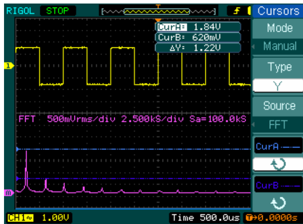
Figure 3-9 Cursor amplitude measurement
