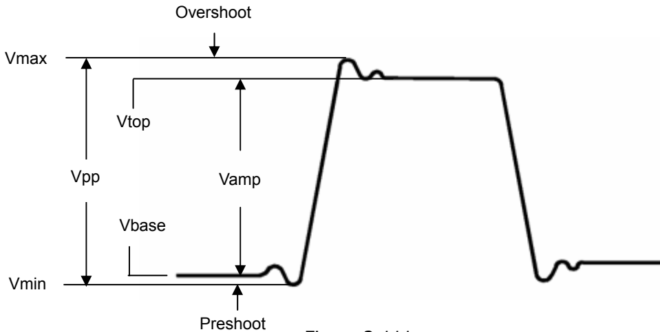
Figure 2-111 Voltage parameters
