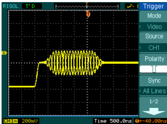
Figure 2-42 Video Trigger: Line Synchronization
