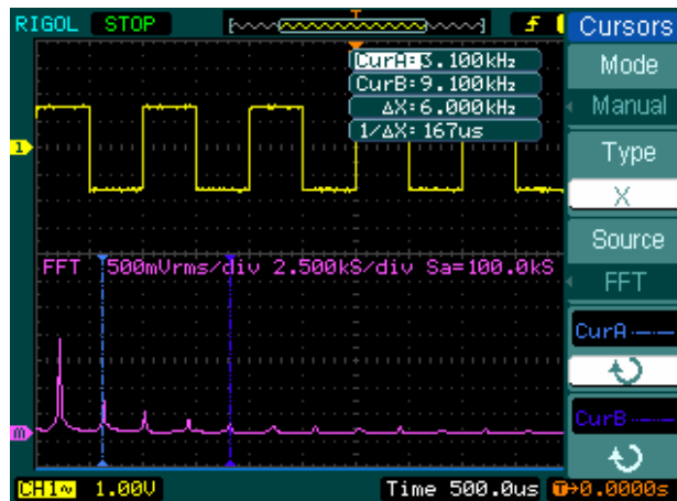
Figure 3-10 Cursor frequency measurement
