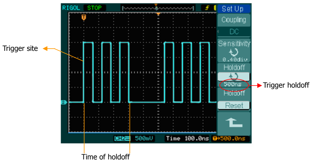
Figure 2-55 Trigger Holdoff
