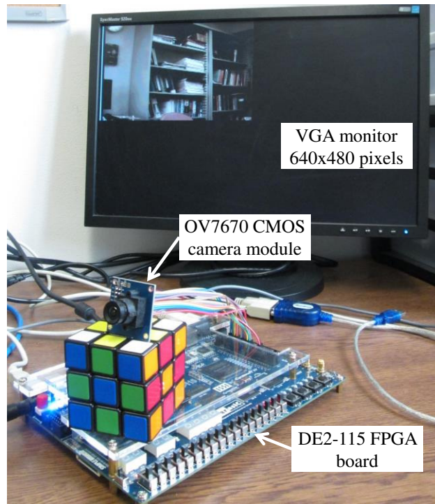
Fig. 3. The experimental setup includes the DE2-115 board that has the OV7670 camera module and a VGA monitor attached to it. Images are captured by the camera and displayed on the VGA display as 320x240 pixel images.
