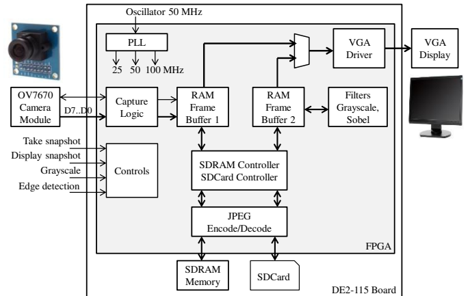
Fig. 1. Block diagram of the proposed baremetal digital camera system.
